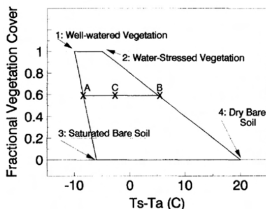
Fig. 1. Illustration of Moran's VIT concept and WDI calculation.
