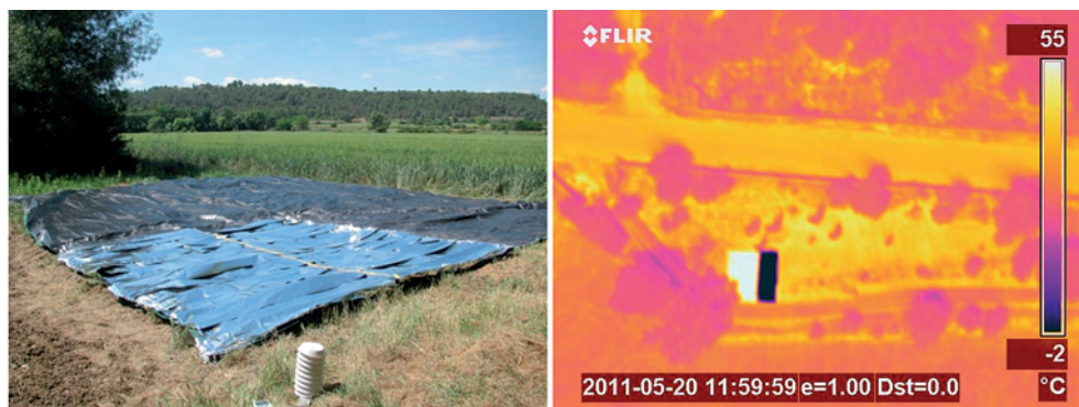
Fig. 12. Example of cold and hot targets on the field and in the thermal image.
