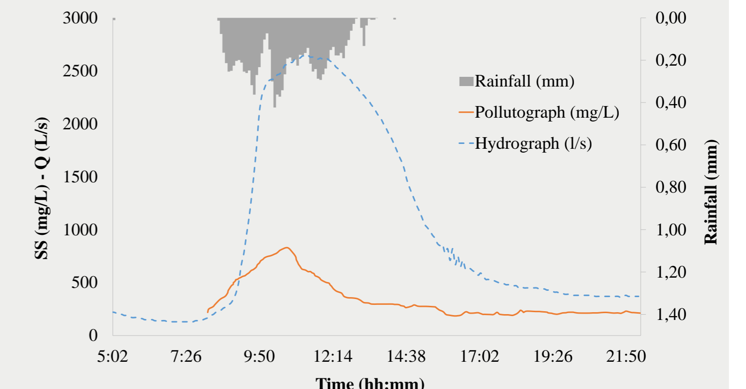
Figure 6: Rainfall, hydrograph and pollutograph of event SF 7.
