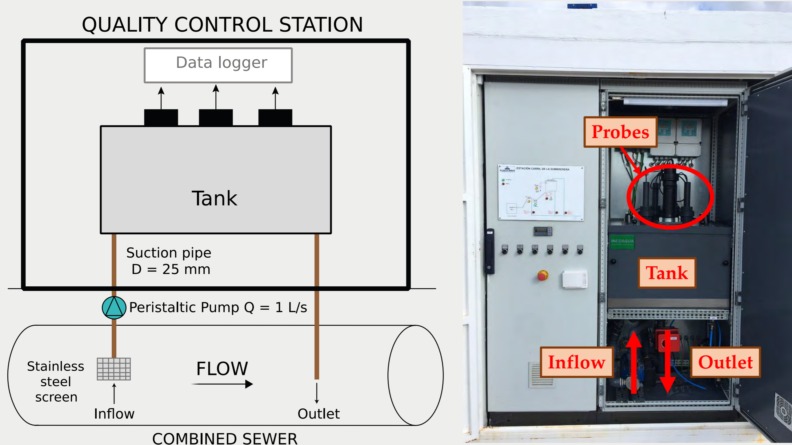
Figure 1: Scheme and image of Quality Control Station devices.
