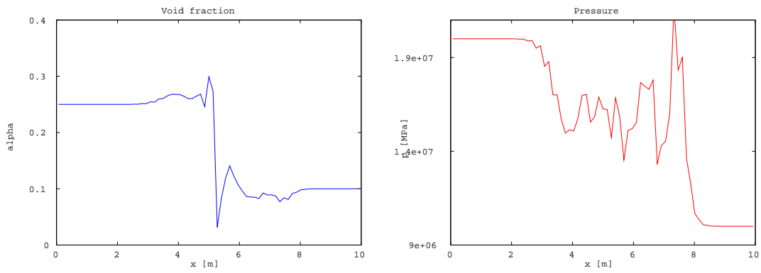
FIGURE 5.3. Results obtained with the ALW scheme for the shock tube problem
