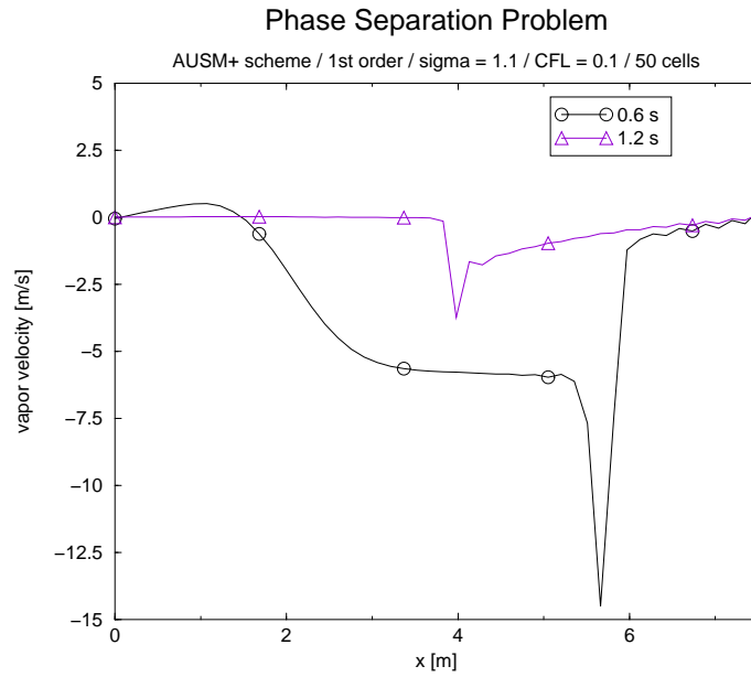
FIGURE 5.41. Vapour velocity
