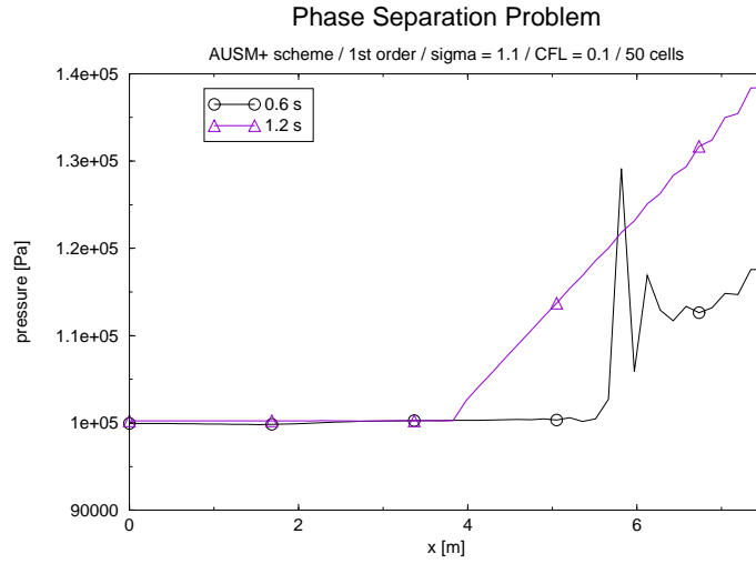
FIGURE 5.40. Pressure
