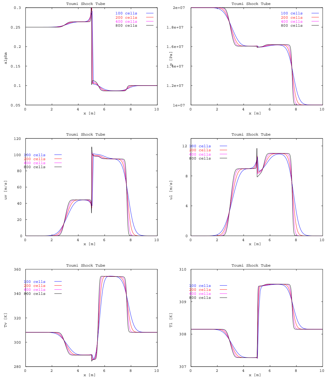
FIGURE 5.17. Toumi's shock tube, 1 st order ATVD: Grid convergence study with the TVD scheme, \sigma = 2.0 . From top to bottom, left to right, void fraction, pressure, gas velocity, liquid velocity, gas temperature, liquid temperature.
