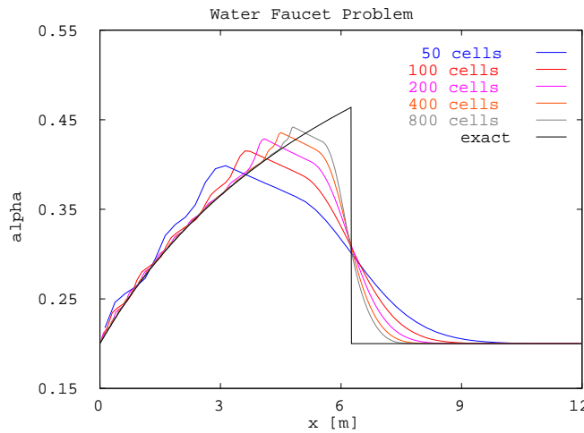
FIGURE 5.14. Grid convergence study for the ATVD scheme
