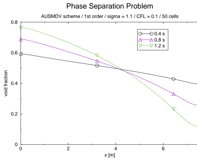
FIGURE 5.44. Void fraction profile for the phase separation test using AUSMDV
