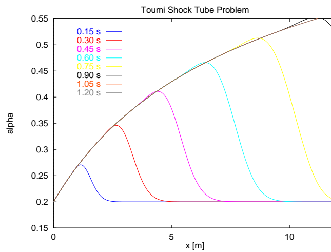
FIGURE 5.26. Evolution of void fraction for a 200 cells mesh
